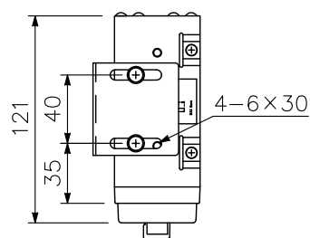
Accessory microphone (1/5)
