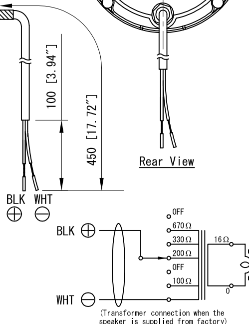
Wiring diagram
